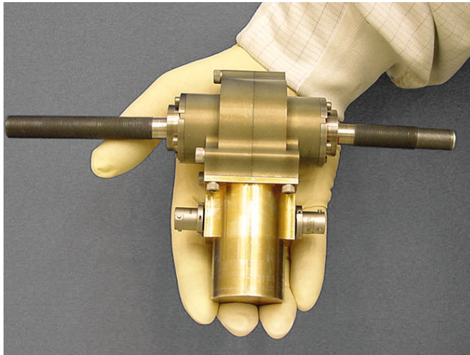
COBD Separation System
