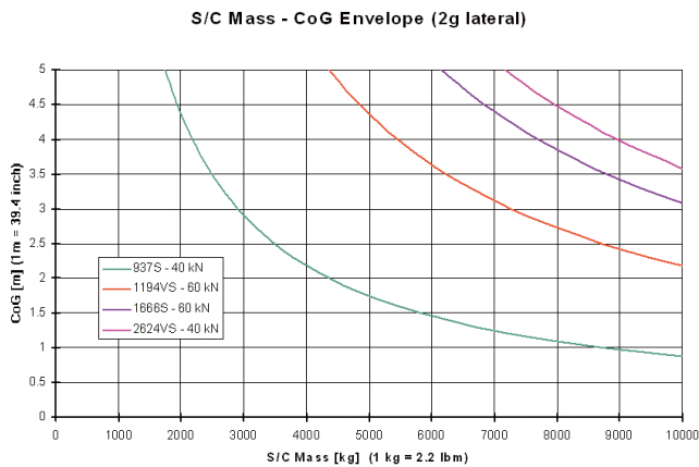
Separation system line load capability
